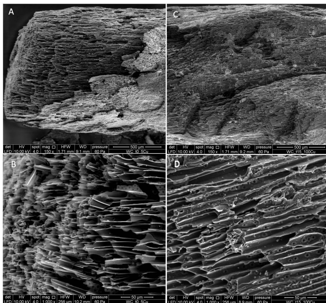
Figure 67 Environmental Scanning Electron Microscopy (ESEM) pictures of fresh, woodchips-derived biochar (A: 150 x magnification; B: 1000 x magnification) and 15 months soil-aged woodchips-derived biochar (C: 150 x magnification; D: 1000 x magnification).
