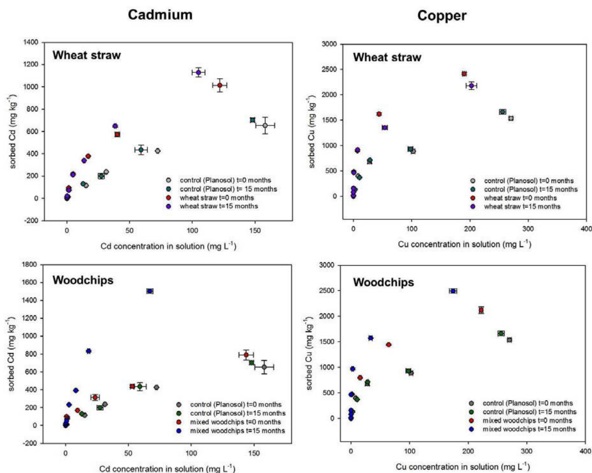
Figure 62 Effects of wheat straw and woodchips derived BC aging in the soil on Cd and Cu sorption behavior (0 and 15 months after start of the pot experiment)
