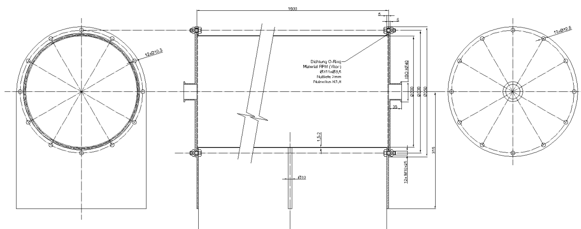
Figure 2: AutoCAD drawing of the pyrolysis furnace
