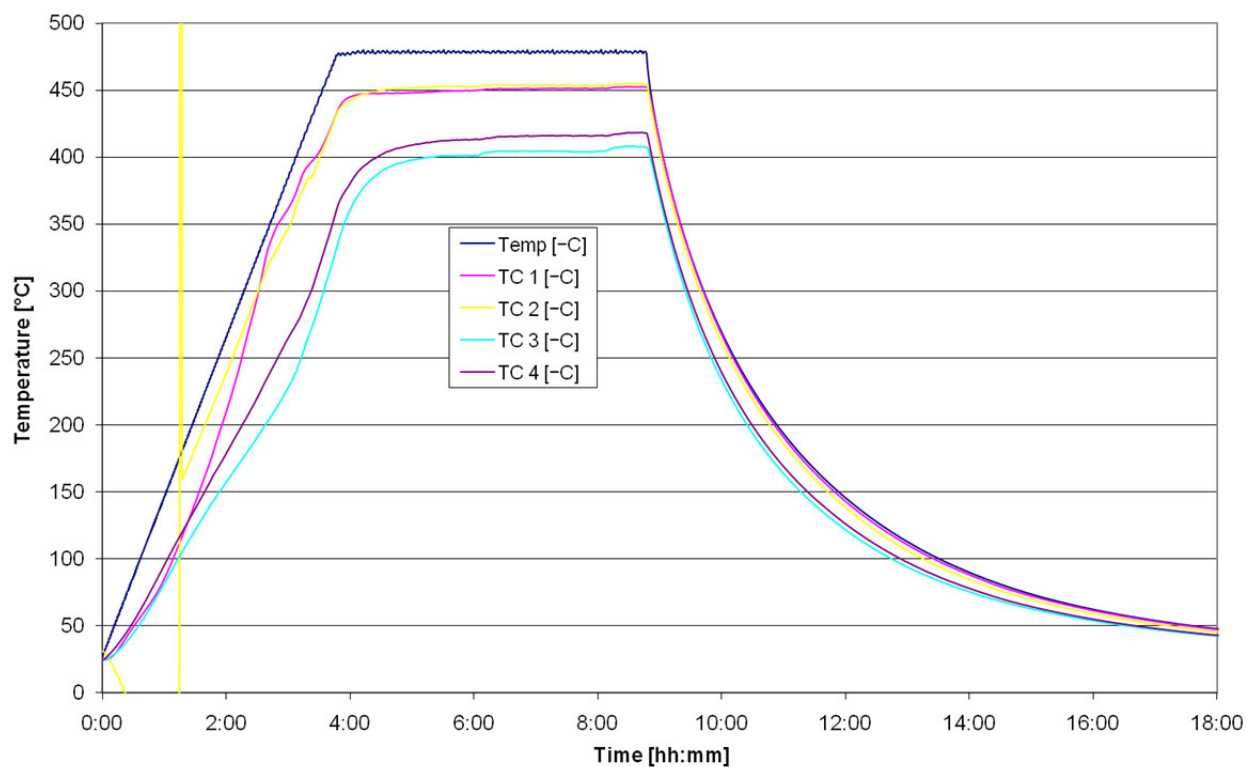
Figure 5: First test run without sample container, straw as feedstock. Heater temp 30 °C above sample temperature inside
