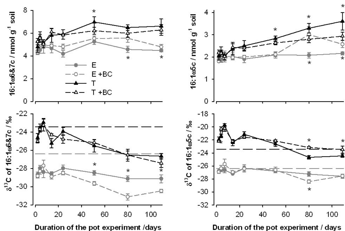
Figure 41: Behaviour of the PLFAs 16:1ω6&7c and 16:1ω5c after 3 % (w/w) biochar application in the pot experiment and their δ¹³C value. Horizontal lines indicate the δ¹³C of the Planosol (grey) and Chernozem (black). Error bars indicate standard deviation (n = 2+2). Significant differences (p ≤ 0.05) are indicated by an asterisk.
