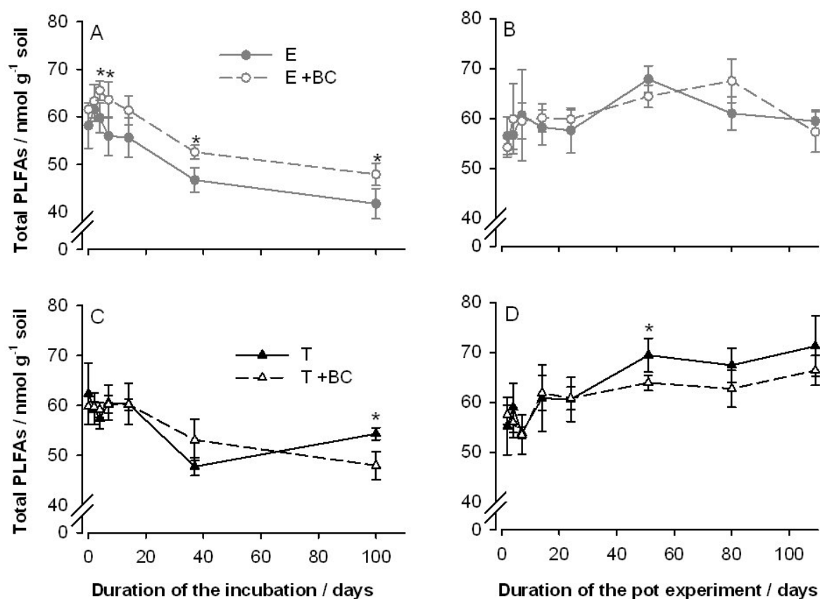
Figure 37: Behaviour of total microbial biomass after 3 % (w/w) biochar application (BC) in the incubation experiment, (A) Planosol and (C) Chernozem, and in the pot experiment, (B) Planosol and (D) Chernozem. Error bars indicate standard deviation (incubation experiment n = 4 ; pot experiment n = 2 + 2 ). Significant differences ( p \leq 0.05 ) are indicated by an asterisk.
