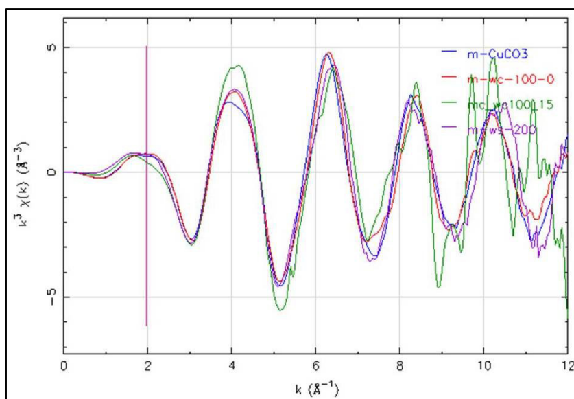
Figure 64 Derivation of EXAFS spectrum (Cu) of fresh (red line) and soil-aged (green line) woodchips-derived biochar
