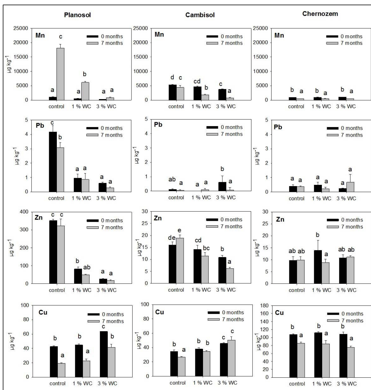
Figure 72 \text{NH}_4\text{NO}_3 extractable trace elements (Mn, Pb, Zn, Cu) of the three investigated soils at 0 and 7 months after start of the pot experiment (WC: woodchips-derived Biochar (BC); 1 and 3 w.-% BC application rate). Statistical evaluation included 2 way ANOVA with the factors BC application rate and sampling time; different letters indicate significant differences at P < 0.05 ; Tukey's post hoc test)
