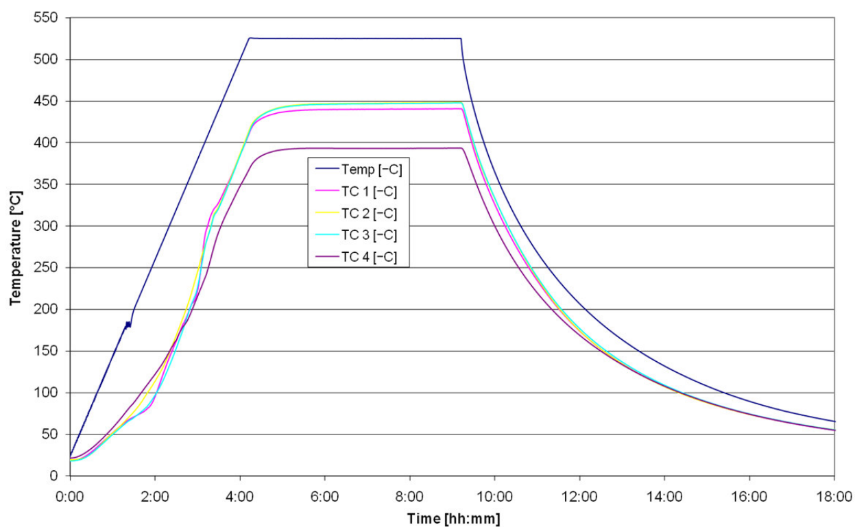
Figure 6: Second test run with sample container, straw as feedstock. Heater temp 75 °C above sample temperature inside
