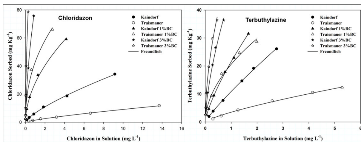
Figure 68 Freundlich adsorption isotherms for chloridazone and terbuthylazine for biochar (BC) treated soils from Kaindorf and Traismauer. 1% BC equals 24 \text{ t ha}^{-1} , 3 % equals 72 \text{ t ha}^{-1} application rate (dry weight).
