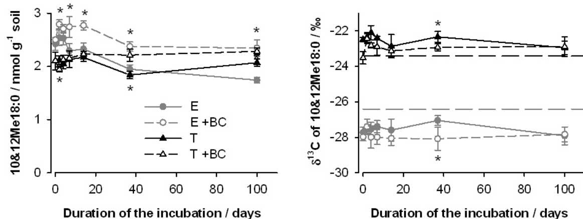
Figure 39: Concentration of the actinomycetal PLFAs 10&12Me18:0 after 3 % (w/w) biochar application in the incubation experiment and its δ 13 C value. Error bars indicate standard deviation (n = 4). Significant differences (p ≤ 0.05) are indicated by an asterisk.
