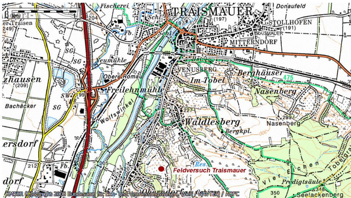
Figure 11: Location of the field experimental site in Oberndorf near Traismauer
