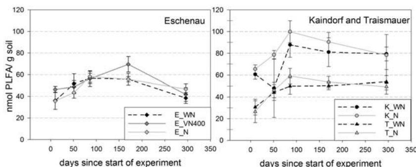
Figure 32: PLFA sums of different treatments with the soil of Eschenau (left) and Kaindorf and Traismauer (right). Error bars indicate standard deviation; n = 5 ; E = Eschenau soil, T = Traismauer soil, W = wood biochar, V400 = vineyard pruning biochar pyrolyzed at 400°C, N = nitrogen fertilizers.
