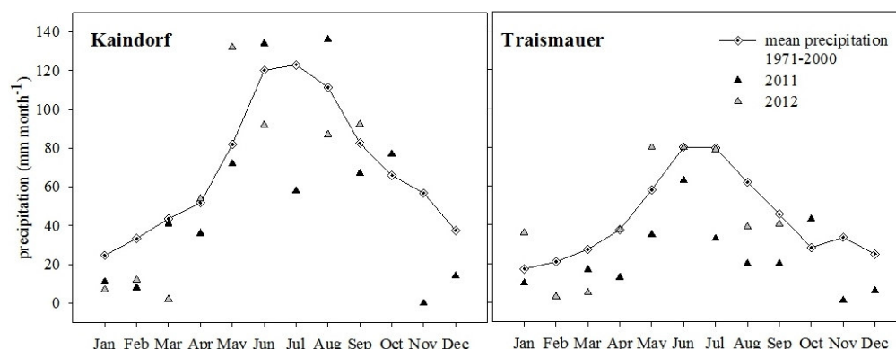
Figure 50 Monthly mean precipitation at the two study sites Kaindorf and Traismauer in 2011 and 2012 compared to the monthly long-term mean precipitation (1971-2000; Karer et al., 2013, Agricultural and Food Science, submitted)
