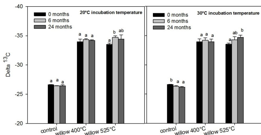
Figure 27 Effect of incubation temperature on ^{13}\text{C} isotopic labeling of soil-biochar mixtures (3 w.-% biochar addition) sampled 0, 6 and 24 months after start of the incubation experiment (Planosol). Different letters indicate significant differences within one treatment ( p < 0.05 ). Numbers behind the treatment indicate the pyrolysis temperature.
