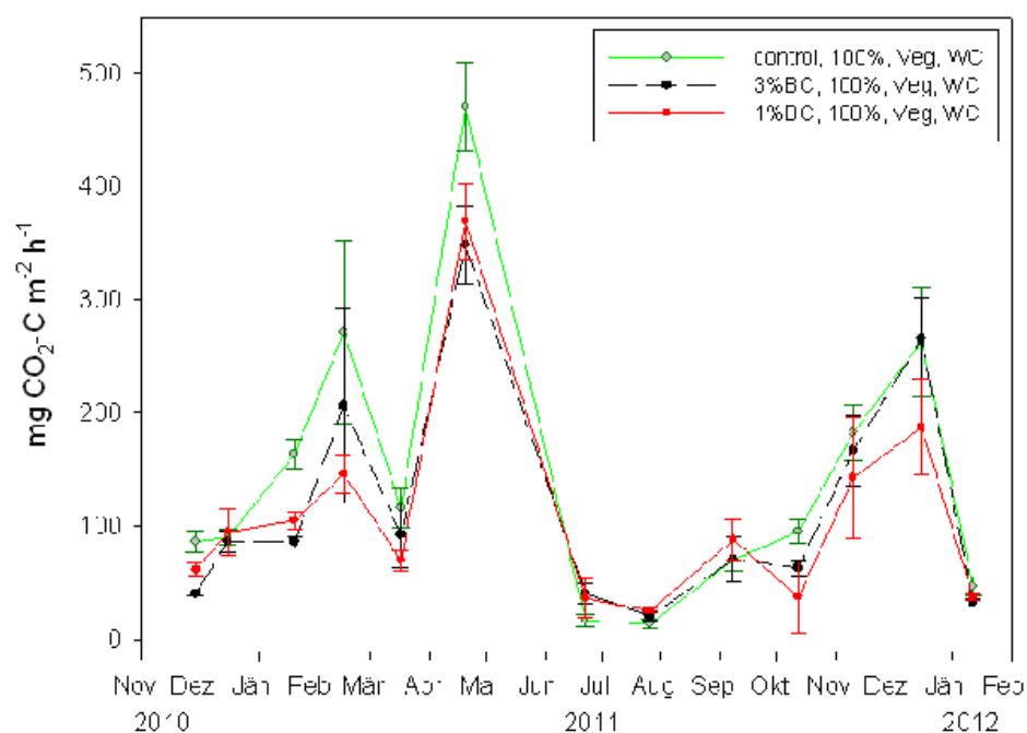
Fig. 1 CO 2 emissions of pots with different biochar treatment (black = 3% biochar, red = 1% biochar, green: no biochar); biochar from wood chips, sandy soil, with vegetation, fertilization rate 100%.
