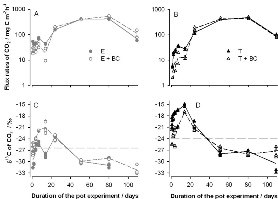
Figure 43: CO 2 emissions (A, B) and δ 13 C value (C, D) emitted from a Planosol (E) and a Chernozem (T) treated with biochar (+BC). Dashed line indicated the δ 13 C value of the Planosol (grey) and Chernozem (black) soil.
