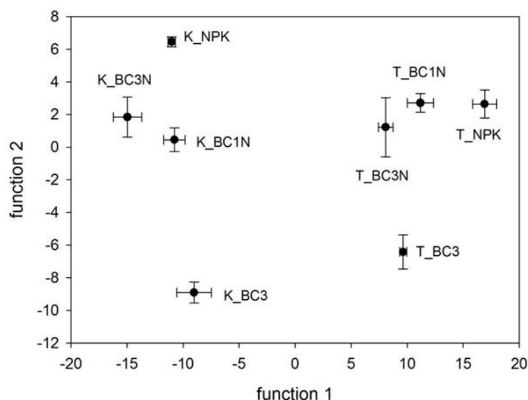
Figure 30: Discriminant function with grouping of various biochars and fertilization treatments from the field experiment. Error bars indicate standard deviation.
