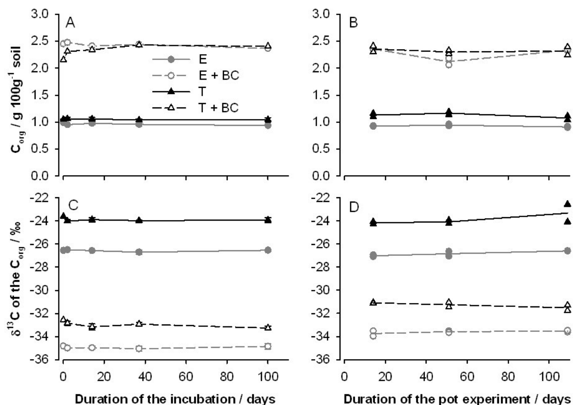
Figure 42: Time behaviour of the soil organic carbon content and its \delta^{13}\text{C} value in the incubation (A and C) and pot (B and D) experiment of the Planosol (E) and Chernozem (T) and amended with 3 % (w/w) biochar (+BC). Error bars in the incubation experiment indicate standard deviation ( n = 4 ).
