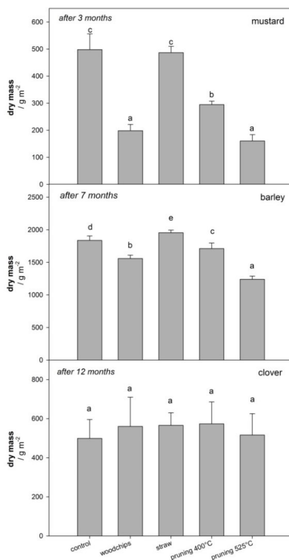
Figure 51 Effect of different biochars on above-ground dry matter production of three successive crops (mustard, barley, clover). Standard fertilization: 40 kg N ha -1 for mustard and 100 kg N ha -1 for barley. Control: standard fertilization without biochar. Different letters indicate significant differences at P < 0.05 (Tukey's post hoc test; n=5 ; Kloss et al., 2013, JPNSS, in review).
