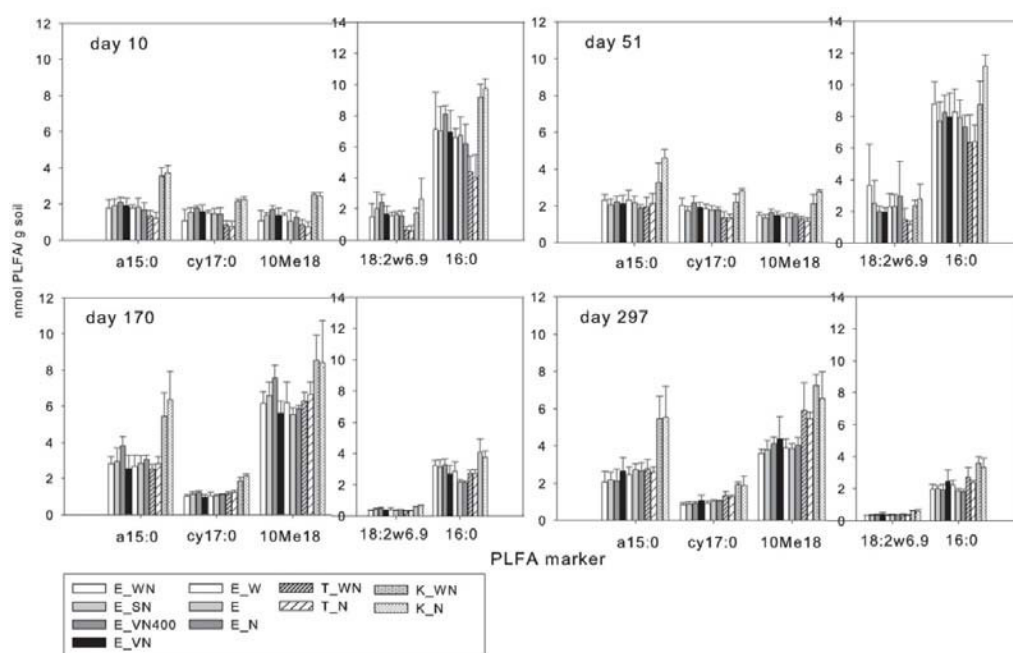
Figure 33: Five PLFAs (a15:0, cy17:0, 10Me18:0, 18:2w6.9 and 16:0) of the treatments on four different sampling days. Error bars indicate standard deviations; n = 5 ; E = Eschenau soil, T = Traismauer soil, W = wood biochar, S = straw biochar, V = vineyard pruning biochar, V400 = vineyard pruning biochar pyrolyzed at 400°C, N = nitrogen fertilizers.
