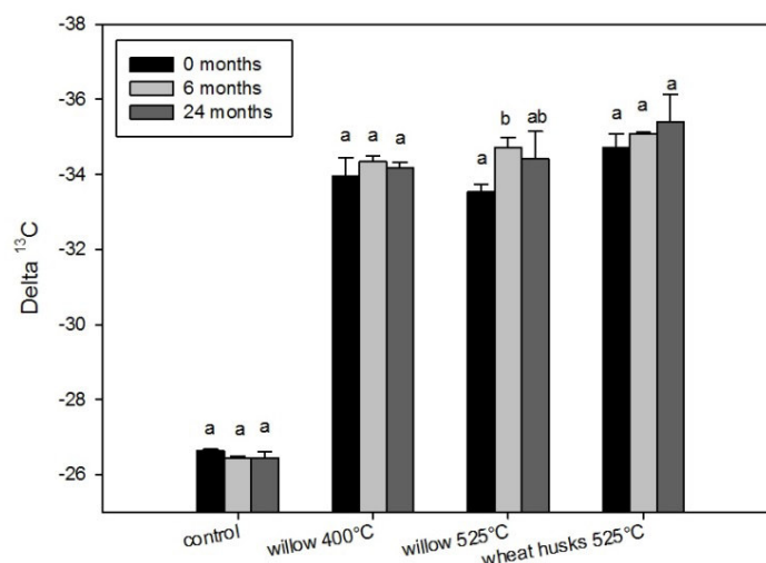
Figure 25 ^{13}\text{C} isotopic labeling of soil-biochar mixtures (3 w.-% biochar addition) sampled 0, 6 and 24 months after start of the incubation experiment (Planosol). Different letters indicate significant differences within one treatment. Numbers behind the treatment indicate the pyrolysis temperature (n=3).
