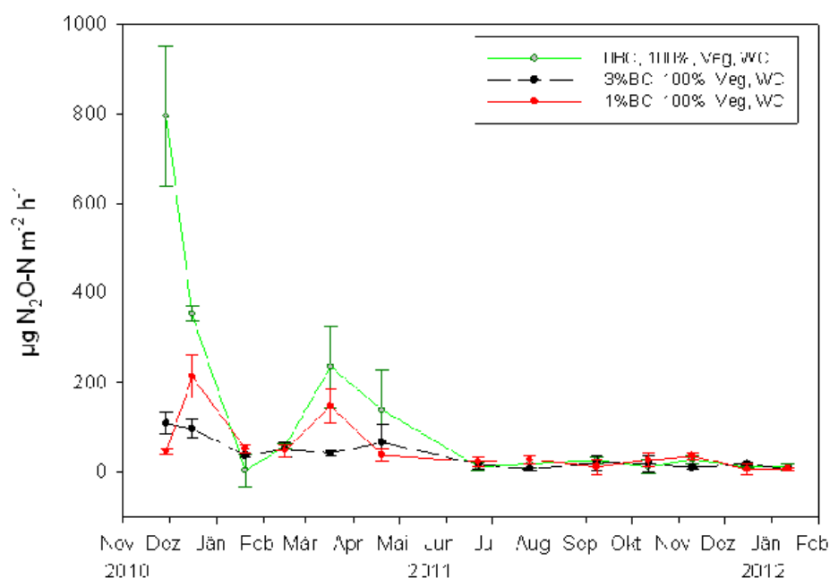
Fig. 4 N 2 O fluxes of different biochar application rates (black = 3%, red = 1%) and control without biochar (green); biochar from wood chips, fertilization rate 100%, sandy soil, with vegetation.
