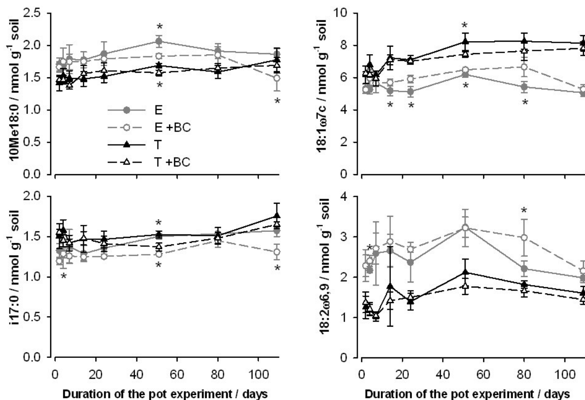
Figure 40: Behavior of single PLFAs representing various microbial groups (actinomycetal PLFA 10Me18:0, Gram negative bacterial PLFA 18:1ω7c, Gram positive bacterial PLFA i17:0 and fungal PLFA 18:2ω6,9) after 3 % (w/w) biochar application (BC) in the pot experiment; E = Planosol and T = Chernozem. Error bars indicate standard deviation ( n = 2 + 2 ). Significant differences ( p \leq 0.05 ) are indicated by an asterisk.
