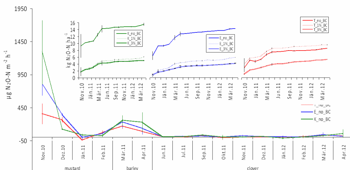
Fig. 2 Pot experiment: Cumulative N 2 O fluxes from control plots and biochar (1% and 3%) treated plots measured at T, E, K and N 2 O emissions of control plots from soils of T, E and K over time.
