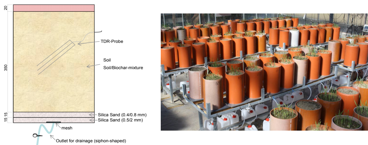
Figure 9: Sketch of one vessel for the pot experiment; lengths in mm (left); set-up of pot experiment in the greenhouse (Photo: J. Bucker)
