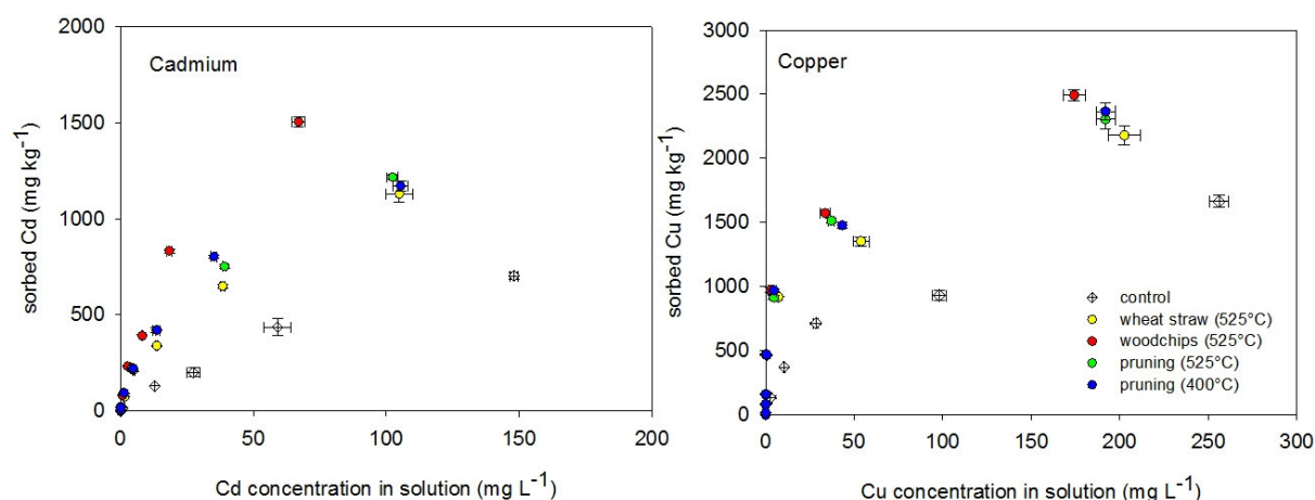
Figure 61 Adsorption isotherm for Cd (left) and Cu (right) for the different biochar treatments (Planosol; 3 w.-% BC application rate; 15 months after start of the pot experiment).
