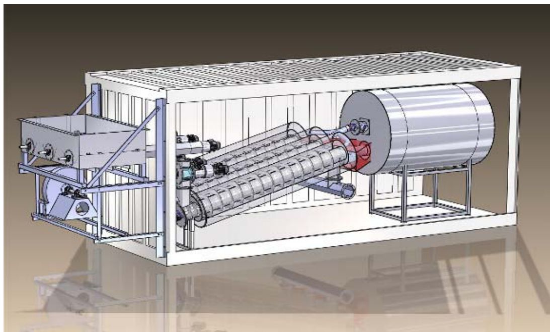
Figure 80: Illustration of the design of the PYREG biochar production plant [PYREG]
