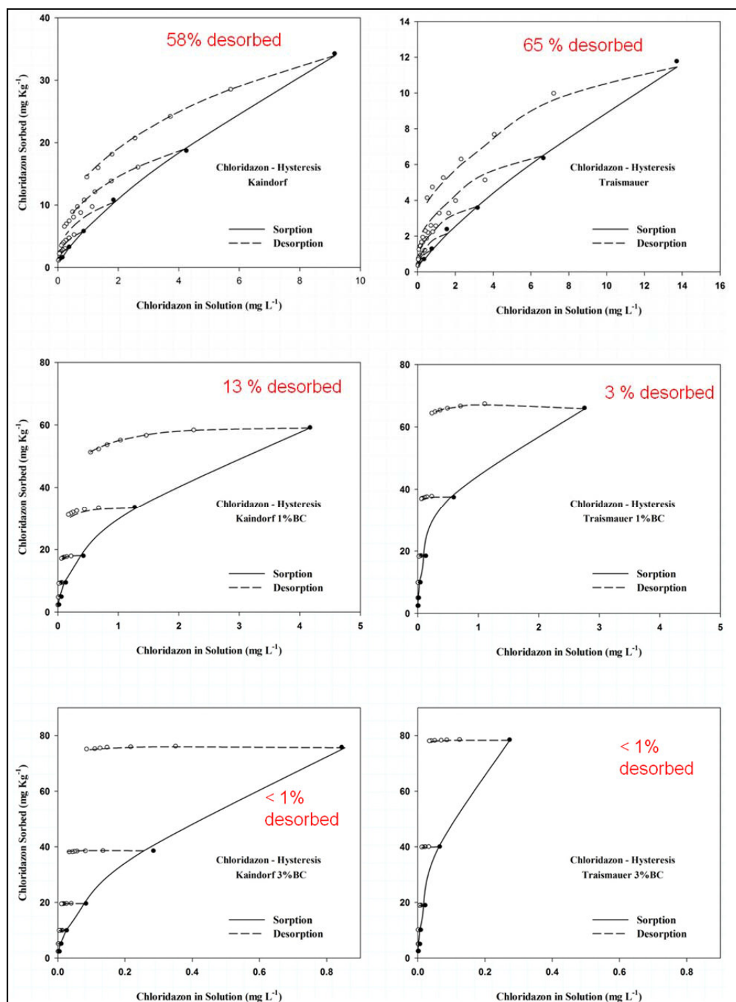
Figure 69 Chloridazone desorption isotherms of the soils with 0, 1 (24 t ha -1 ) and 3 (72 t ha -1 ) w.-% BC application for Kaindorf (left column) and Traismauer (right column).
