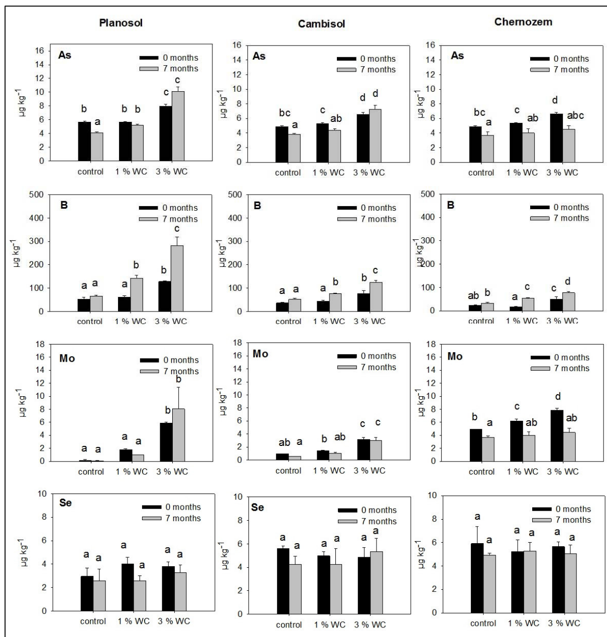
Figure 73 \text{NH}_4\text{NO}_3 extractable trace elements (As, B, Mo, Se) of the three investigated soils at 0 and 7 months after start of the pot experiment (WC: woodchips-derived Biochar (BC); 1 and 3 w.-% BC application rate). Statistical evaluation included 2 way ANOVA with the factors BC application rate and sampling time; different letters indicate significant differences at P < 0.05 ; Tukey's post hoc test).
