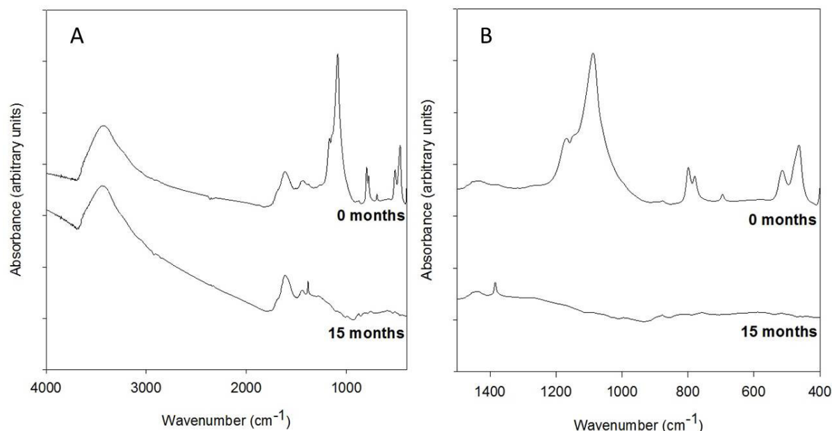
Figure 66 Fourier-Transform Infrared Spectroscopy (FTIR) spectra of fresh (0 months) and soil-aged (15 months) Woodchips-derived biochar. One increment of the y-axis corresponds to 0.1 absorbance units ( n=1 ). A) Full spectra from 4000 to 400 \text{cm}^{-1} ; B) fingerprint region from 1500 to 400 \text{cm}^{-1} .
