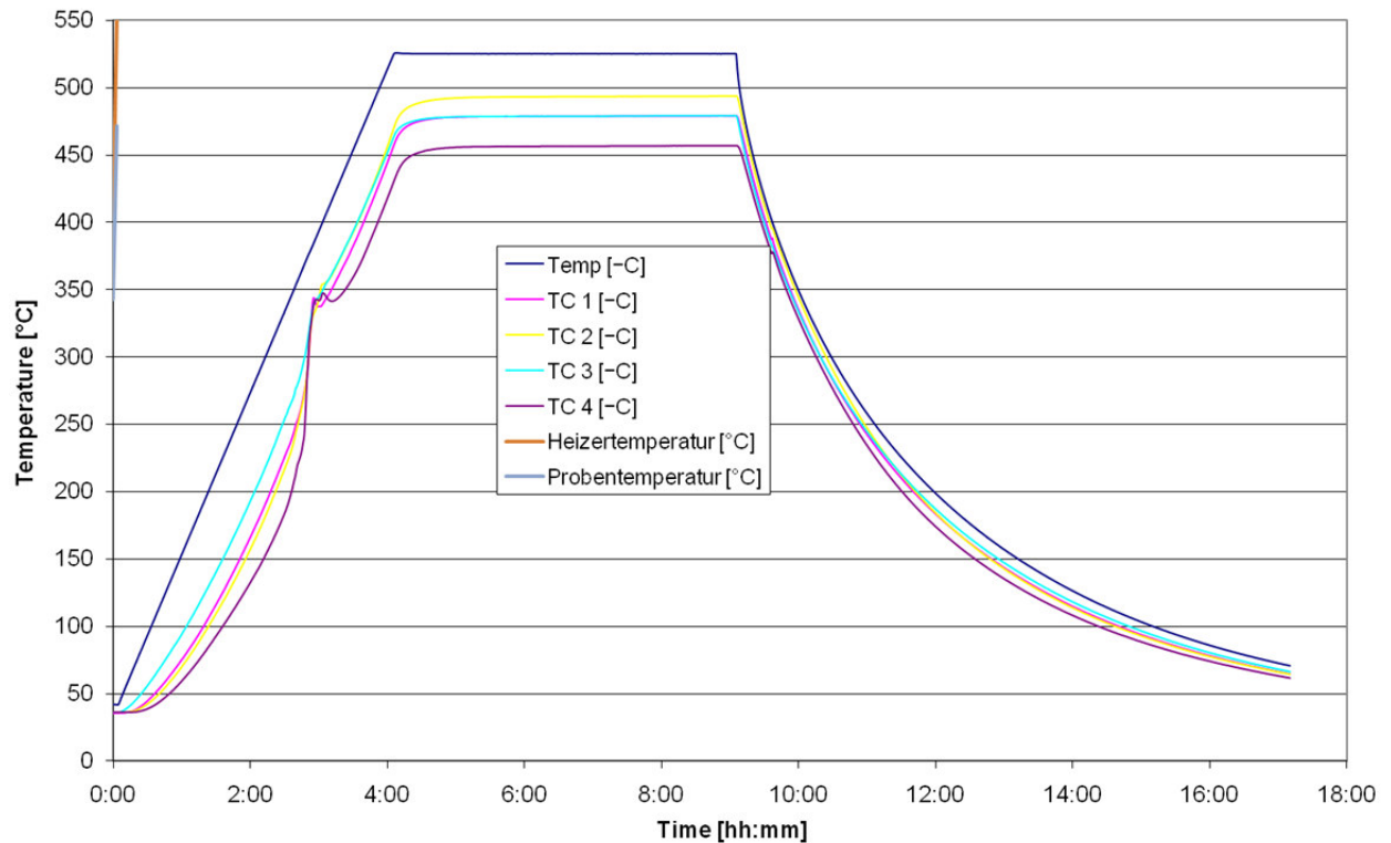
Figure 7: Third test run with sample container, vine wood as feedstock. Heater temp 45 °C above sample temperature inside
