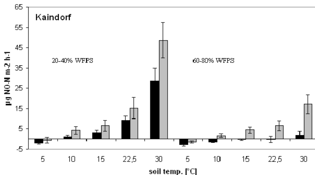
Fig. 6 Nitric oxide fluxes at dry (20-40% WFPS) and wet soil (60-80% WFPS) under different soil temperatures at the site Kaindorf. Black bars=biochar treated, grey bars=control.
