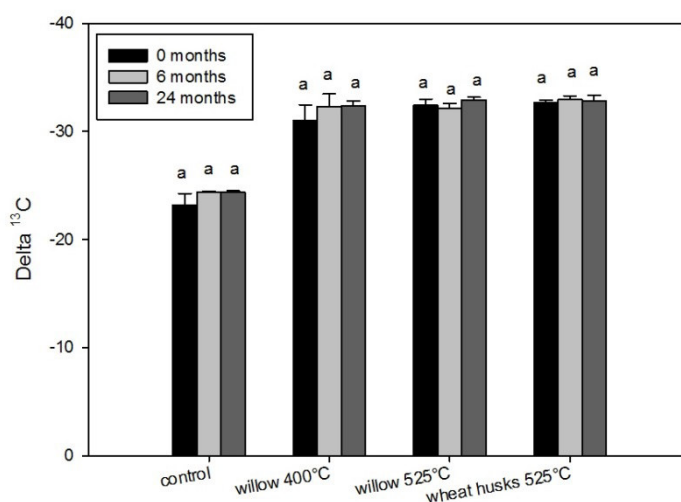
Figure 26 ^{13}\text{C} isotopic labeling of soil-biochar mixtures (3 w.-% biochar addition) sampled 0, 6 and 24 months after start of the incubation experiment (Chernozem). Different letters indicate significant differences within one treatment. Numbers behind the treatment indicate the pyrolysis temperature (n=3).
