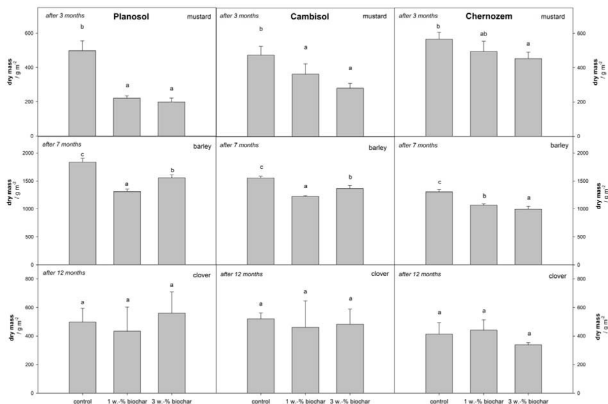
Figure 52 Effect of different biochar application rates on above-ground dry matter production of three successive crops (mustard, barley, clover) on three different agricultural soils (Planosol, Cambisol, Chernozem). Different letters indicate significant differences at P < 0.05 (Tukey's test; n=5 ; Kloss et al., 2013, JPNSS, in review).
