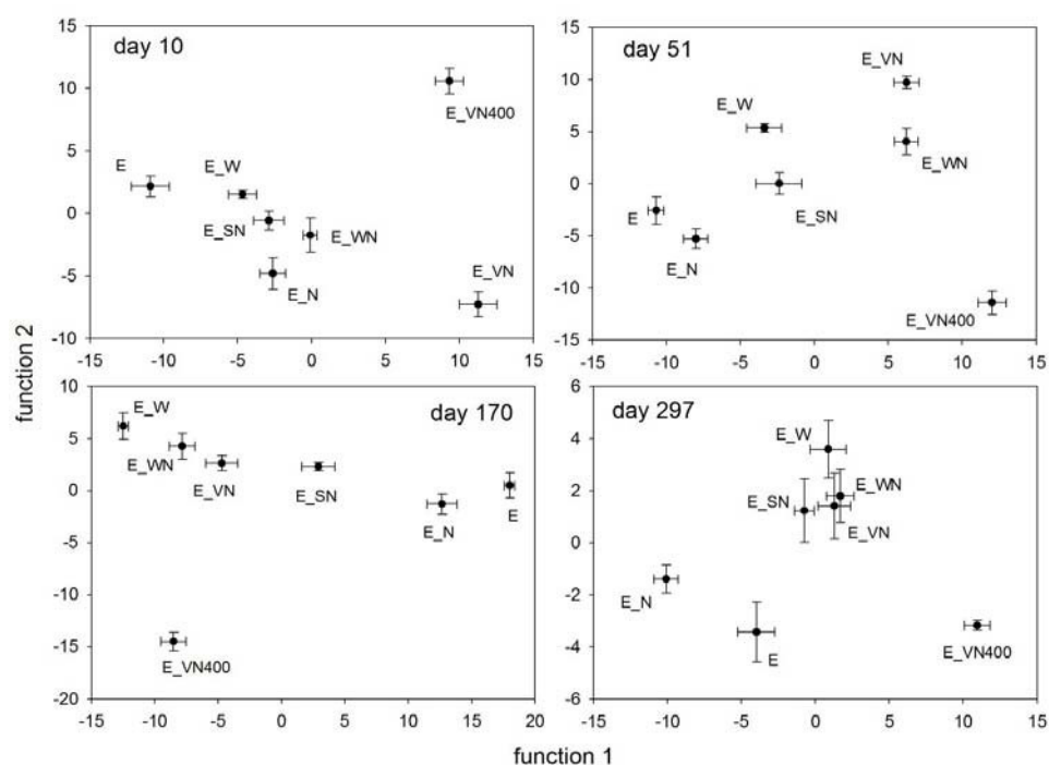
Figure 34: Discriminant functions with grouping of various biochar and fertilization treatments for Eschenau. Error bars indicate standard deviation. E = Eschenau soil, T = Traismauer soil, W = wood biochar, S = straw biochar, V = wineyard pruning biochar, V400 = wineyard pruning biochar pyrolyzed at 400°C, N = nitrogen fertilizers.
