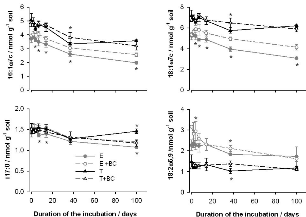
Figure 38: Behavior of the single PLFAs representing various microbial groups (Gram negative bacterial PLFAs 16:1ω7c and 18:1ω7c, Gram positive bacterial PLFA i17:0 and fungal PLFA 18:2ω6,9) after 3 % (w/w) biochar application (BC) in the incubation experiment; E = Planosol and T = Chernozem. Error bars indicate standard deviation (n = 4). Significant differences (p ≤ 0.05) are indicated by an asterisk.
