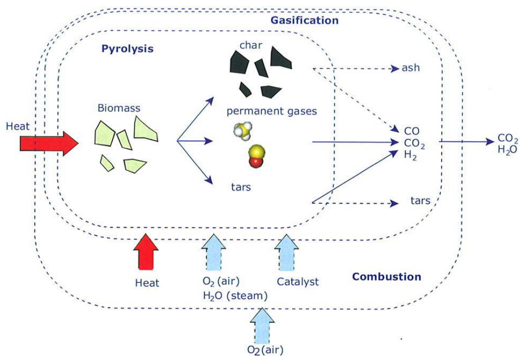
Figure 77: Schematic description of biomass decomposition [Knoef 2005]
