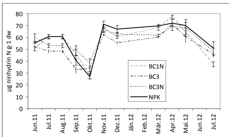
Fig. 10 Nmic from BC treated and control plots at the field site Traismauer over time.
