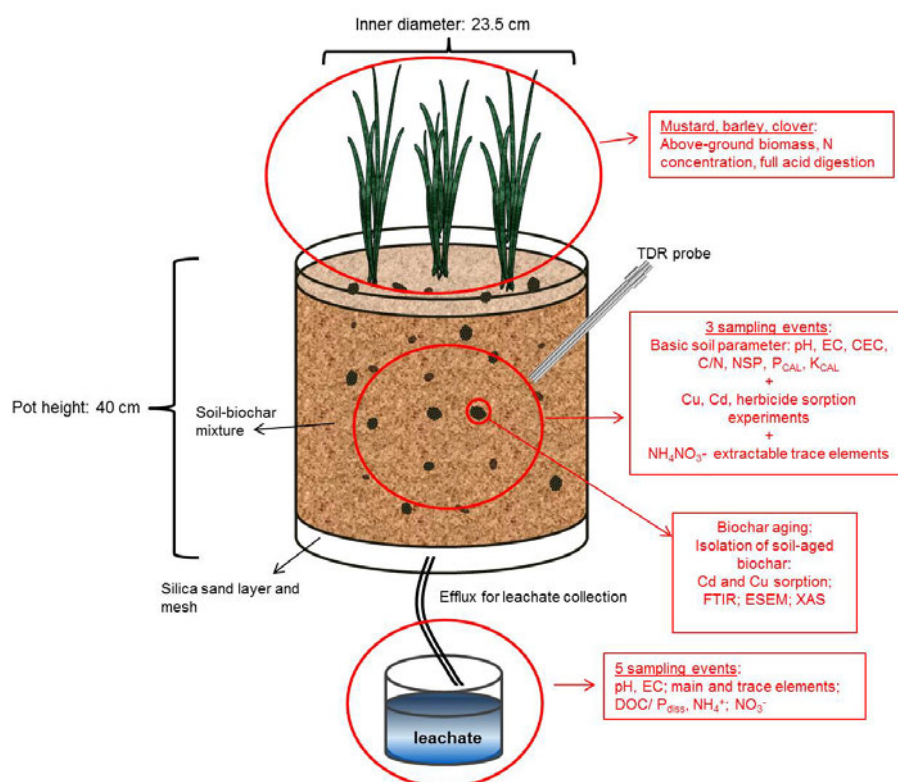
Figure 48 Scheme of the dimensions of a pot from the glasshouse experiment and realized analyses within the work package 5 (red boxes). EC: electrical conductivity; CEC: cation exchange capacity; NSP: nitrogen supplying potential; P_{CAL}/K_{CAL} : calcium-acetate-lactate extractable phosphorus and potassium; FTIR: Fourier-Transform Infrared Spectroscopy; ESEM: Environmental Scanning Electron Microscopy; XAS: X-ray absorption spectroscopy; DOC: dissolved organic carbon; P_{diss} : dissolved phosphorus.
