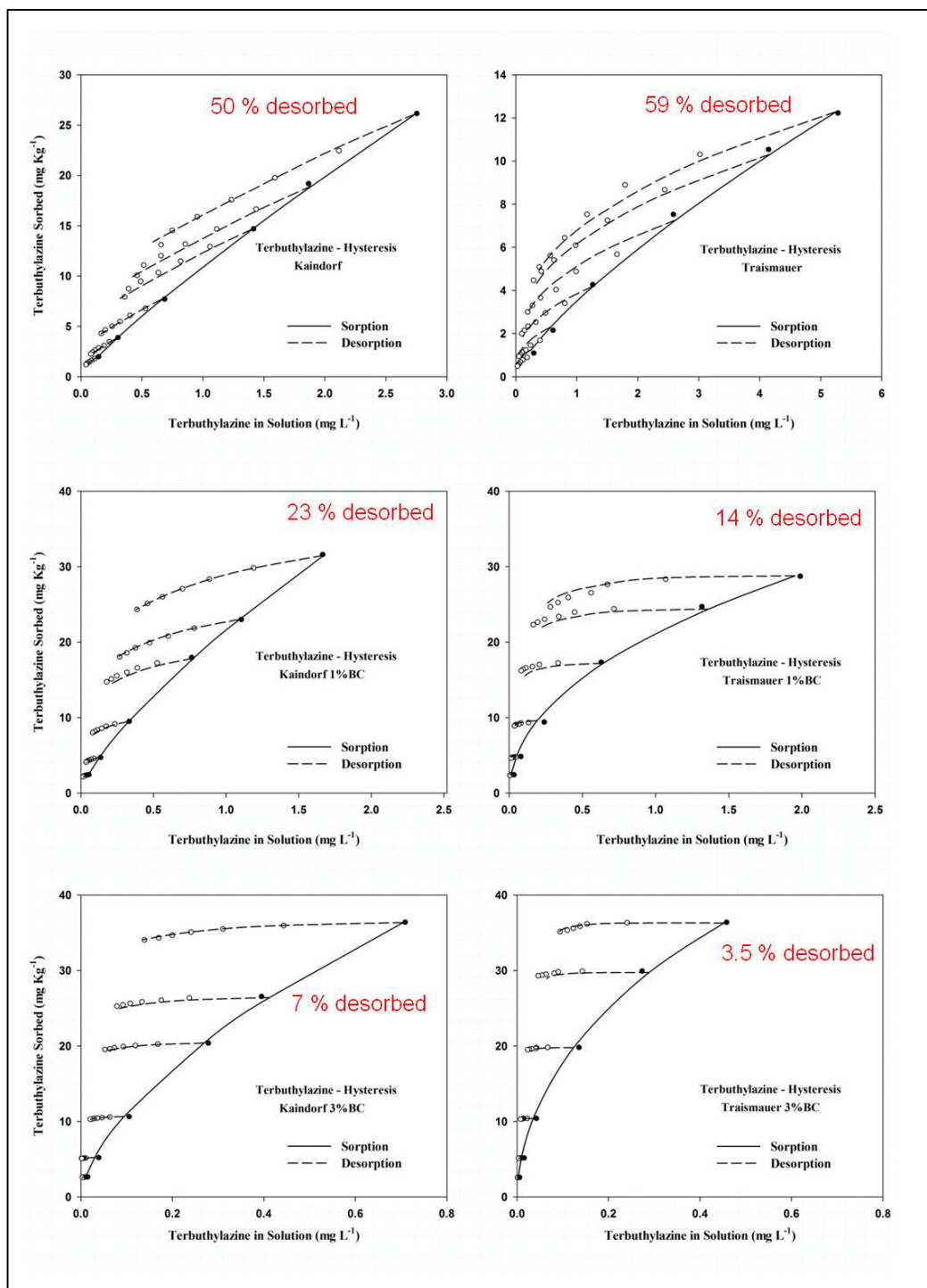
Figure 70 Terbutylazine desorption isotherms of the soils with 0, 1 ( 24 \text{ t ha}^{-1} ) and 3 ( 72 \text{ t ha}^{-1} ) w.-% BC application for Kaindorf (left column) and Traismauer (right column).
