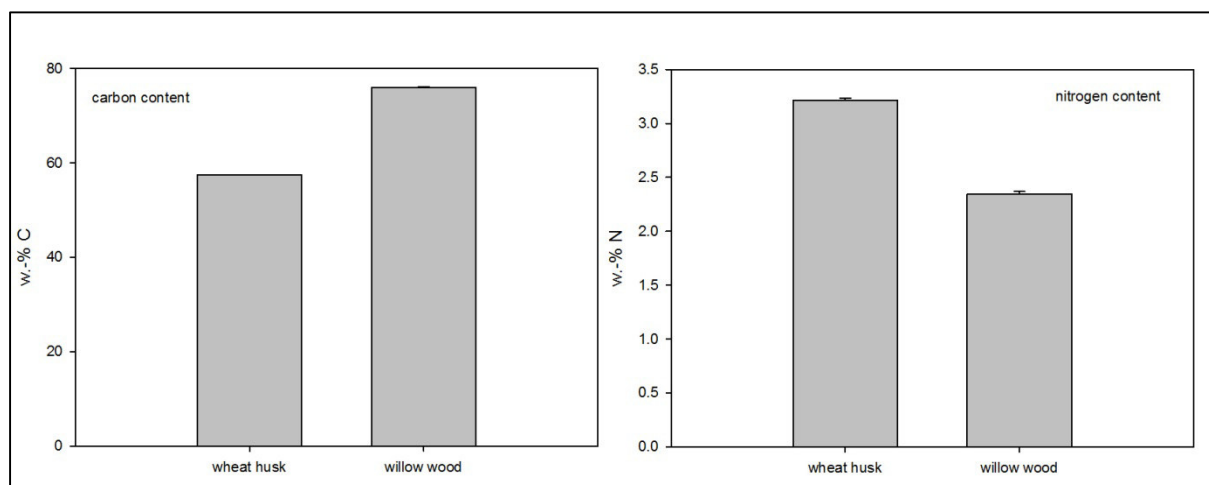
Figure 21 C and N content of wheat husk and willow wood derived biochar (525°C pyrolysis temperature; n=3).
