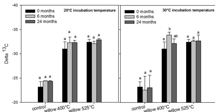
Figure 28 Effect of incubation temperature on ^{13}\text{C} isotopic labeling of soil-biochar mixtures (3 w.-% biochar addition) sampled 0, 6 and 24 months after start of the incubation experiment (Chernozem). Different letters indicate significant differences within one treatment ( p < 0.05 ). Numbers behind the treatment indicate the pyrolysis temperature.
