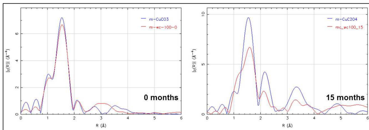
Figure 65 EXAFS spectra (Cu) of fresh (left picture) and aged (right picture) BC in relation to Cu speciation.
