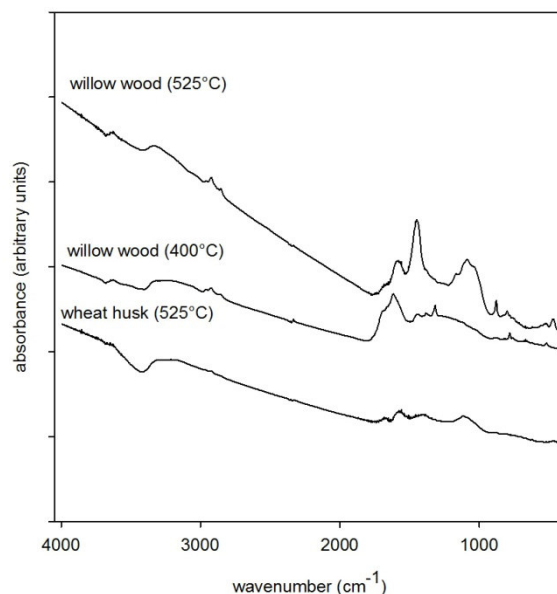
Figure 22 FTIR spectra of the 13 C labeled biochar used for the incubation experiment. Respective pyrolysis temperatures are given in brackets.
