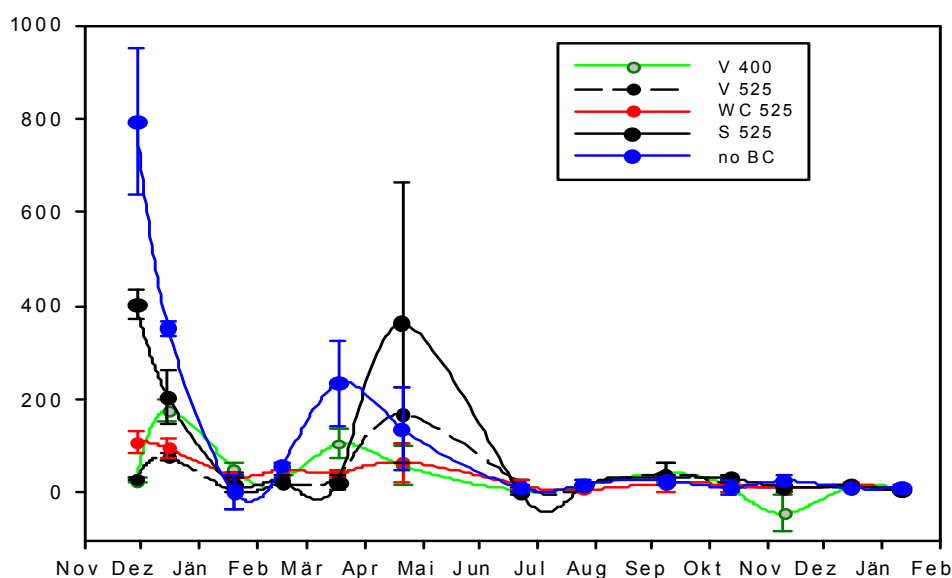
Fig. 5 \text{N}_2\text{O} fluxes of different types of biochar (BC) (green = BC from vineyard pruning, pyrolysis temperature 400^\circ\text{C} ; black, dotted line = BC from vineyard pruning, pyrolysis temperature 525^\circ\text{C} ; red = BC from wood chips, pyrolysis temperature 525^\circ\text{C} ; black, full line = BC from straw, pyrolysis temperature 525^\circ\text{C} ; blue = control without biochar application), sandy soil, with vegetation, fertilization rate 100%.
